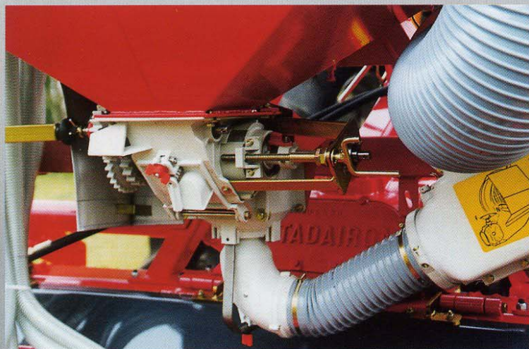
Calibrating system - Accurate calibration
